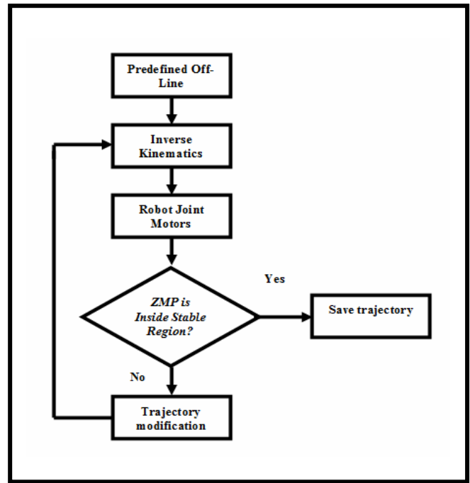
Figure1. Block diagram of the first phase
